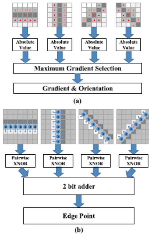
Fig. 4. Directional pairwise edge detection. (a) Edge detection method in [25]. (b) Edge point detection method in this work.
