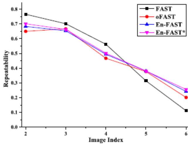
Fig. 7. Repeatability comparison (En-FAST* with DPED enabled only).
