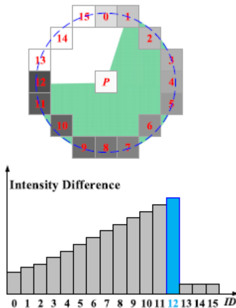
Fig. 5. Score and orientation estimation methods.
