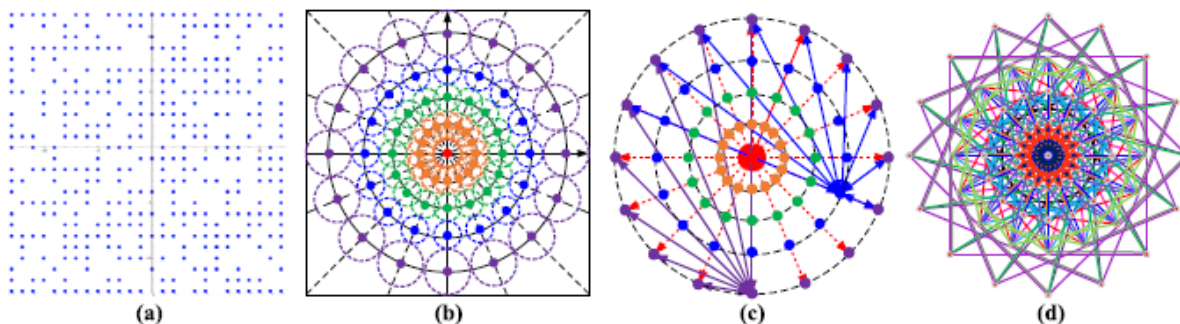
Fig. 6. Different sampling patterns and L-BIRD sampling pairs. (a) ORB. (b) L-BIRD. (c) Sampling pair selection approaches and constraints. (d) Sampling pattern of a 256-bit L-BIRD descriptor.
