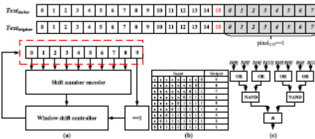
Fig. 11. (a) STU. (b) Truth table of shift number encoder. (c) Early rejection. if the next bit is 0. Otherwise, the window head is shifted to the last bit of 1 appeared in the window equality check. The start position is the window head position if the window equality check is successful. The end position is decided until the first 0 appeared in the following bits of the text. As proved in [20], the case of keypoint test is always ended earlier than the cases of nonkeypoint test. However, most of the pixels in regular images are not keypoints. Therefore, some early termination methodologies should be developed to end the segment test as soon as possible if the candidate pixel is not a keypoint. In this paper, a similar early rejection approach, which considers four pixel values at 0, 4, 8, and 12, is also proposed to terminate the segment test simultaneously. Considering the special scenario of the proposed segment test, the candidate pixel is rejected only when two zeroes exist in both the two 16-bit strings. The detailed
