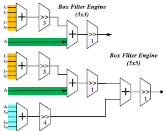
Fig. 13. BFE implementation.
