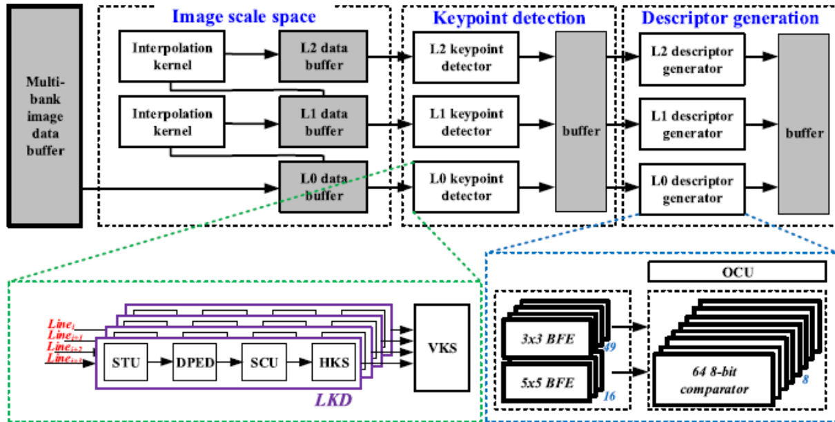
Fig. 9. System architecture of the accelerator.
